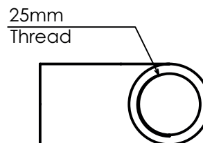
Left view
