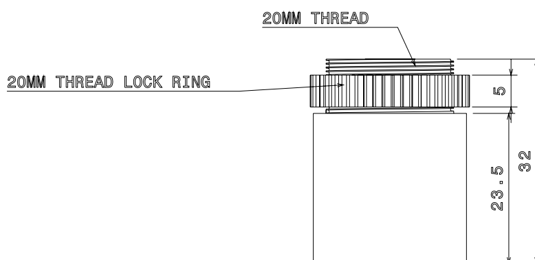
side view
