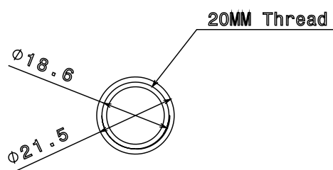
Bottom view
