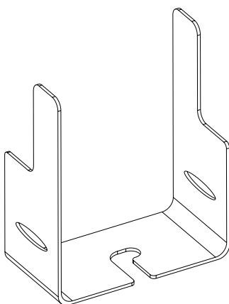
Isometric view
